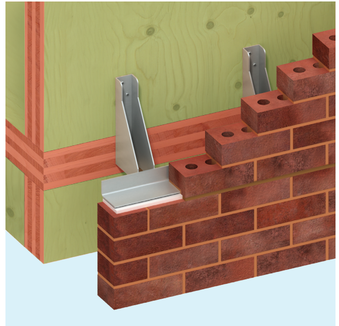
M8 x 100mm washer head SPAX screws should only be fixed into the areas shown in green. Areas shown in red i.e. ends of walls or floor panels should not be fixed into.
