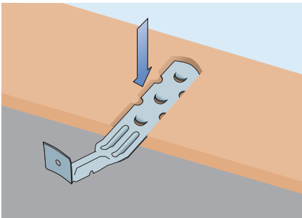
Wall ties should be pressed down in, and then surrounded by, fresh mortar.
