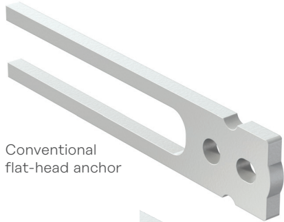
Clutch shear load deforms the anchor to the side.
