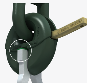
EPNA systems have more distance between the clutch and anchor sides which increases shear resistance.
