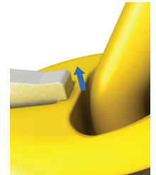
Rotation causes the side of the clutch to bear against the top of the anchor causing a shearing force to the side.
