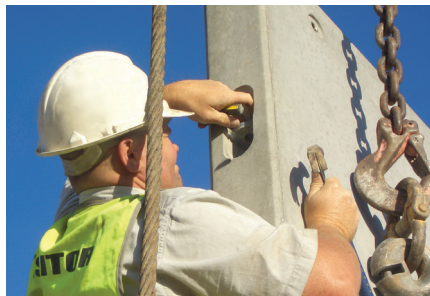
On-site maintenance work required to clean lifting holes
