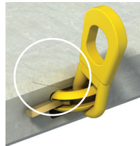
Anchor bearing crack
