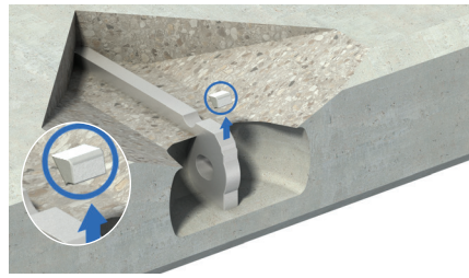
Anchor sheared by the clutch
