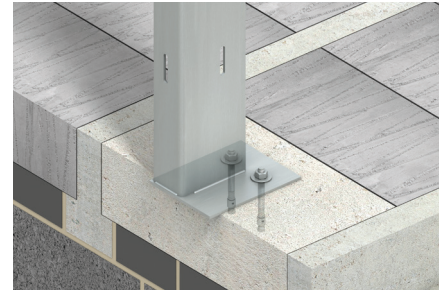
Base Connection of a WP2 Windpost to a Concrete Infill in the Top of a Beam and Block Floor
