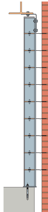
WP2 Windpost Fixed to Top of Concrete and Underside of Steel Beam
