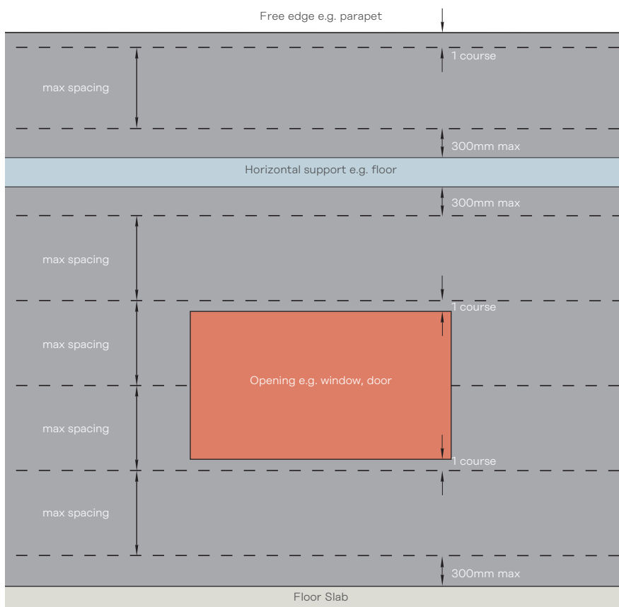
Masonry Reinforcement
