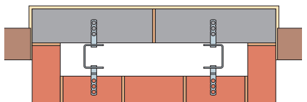
WP3 Windposts with SDN and SPN Ties Providing Support for Brick Pier
