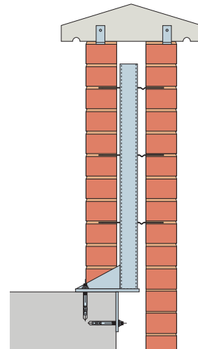
WP3 Parapet Post Fixed to Top and Face of Concrete
