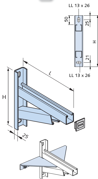
Assembly example with bracing KON Z1 (see below)
