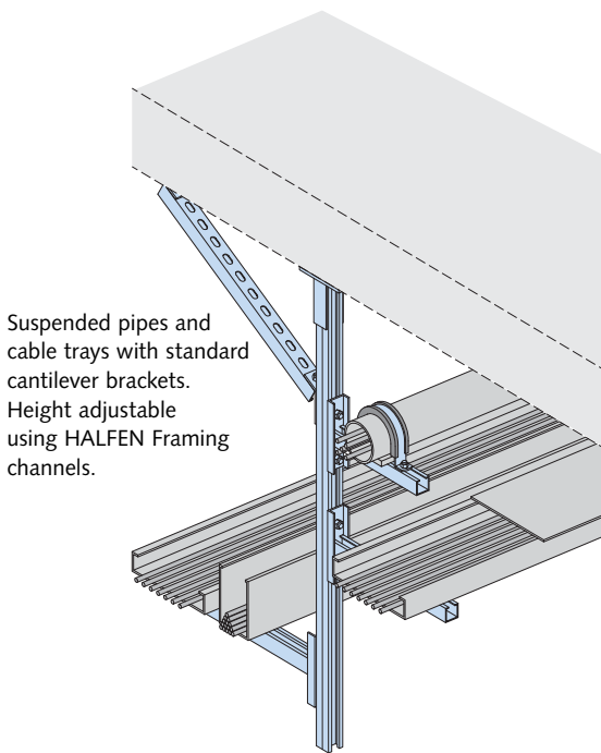
HALFEN Adjustable cantilever Angle and height adjustable
