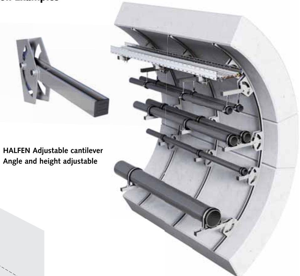
HALFEN Cantilever height adjustable
