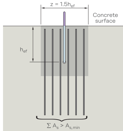
Reinforcement Details
