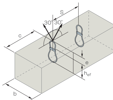
Transverse Installation
