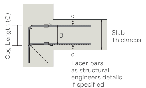
Schematic figure of a double-row LL-type Coupler Box within a slab-to-wall connection
