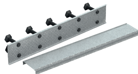
Ancon KSN Anchor Box using Ancon KSN Anchors with Ancon BT Starter Bars
