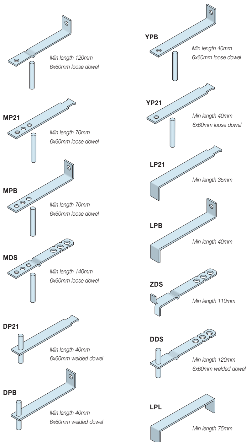
Ancon LDB Ties Fixed to Backing Structure, Restraining Top of Stone
