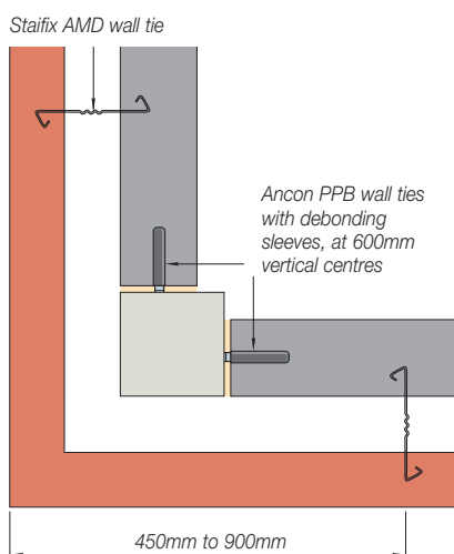
External Corner with Fully Bonded Brickwork
