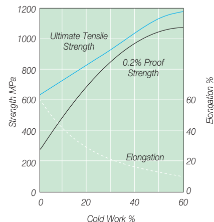
Effect of Cold Working in Grade 304 Stainless Steel
