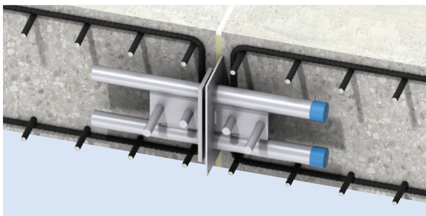
DSD Shear Load Connector
