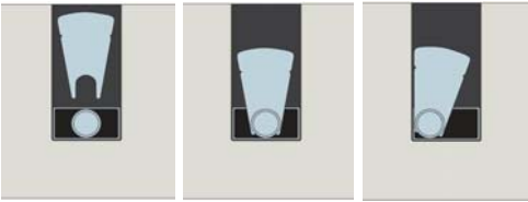
The fan-shaped Locking Plate allows the dowel to be locked in any position.
