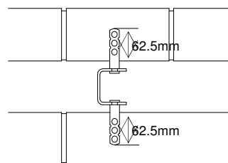
TIE EMBEDMENT (WP1/WP3)
